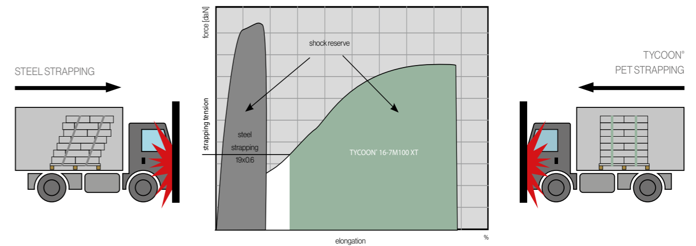
The shock reserve is a combination of elongation and breaking strength.
