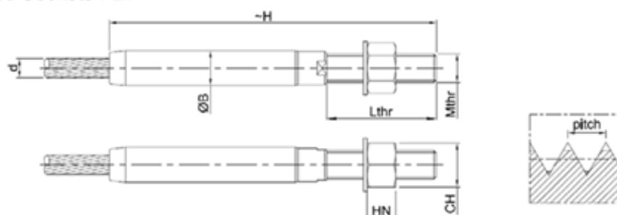
SWAGED FITTING - 42CrMo4 (1.7225 EN ISO 683-2:2008) see Annex B
